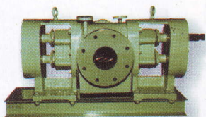
External bearing type gear pump with jacket
